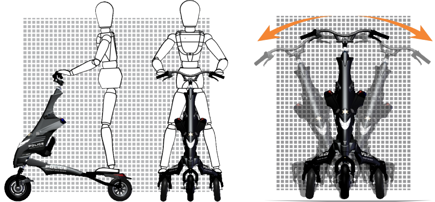
CAMBERING VEHICLE
